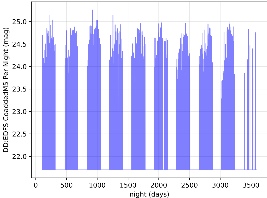
ddf_loaded_half_fl2_v3.4_10yrs z band: DD:EDFS CoaddedM5 Per Night
