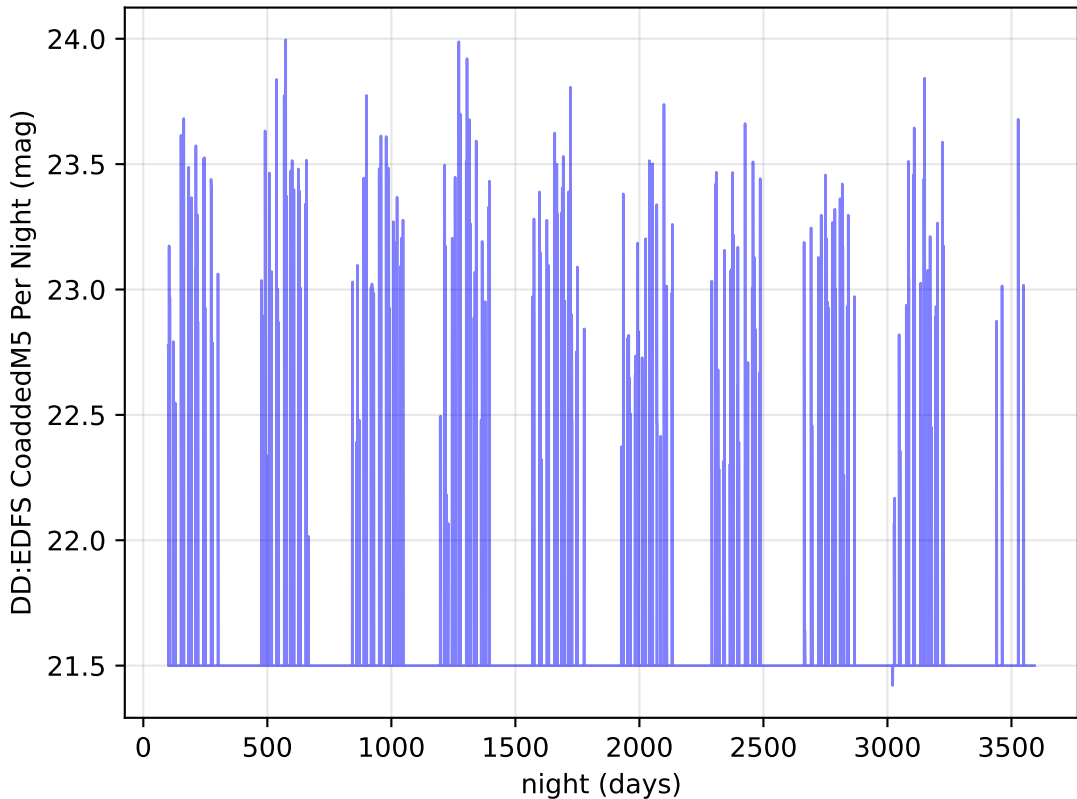
ddf_loaded_half_fl2_v3.4_10yrs y band: DD:EDFS CoaddedM5 Per Night
