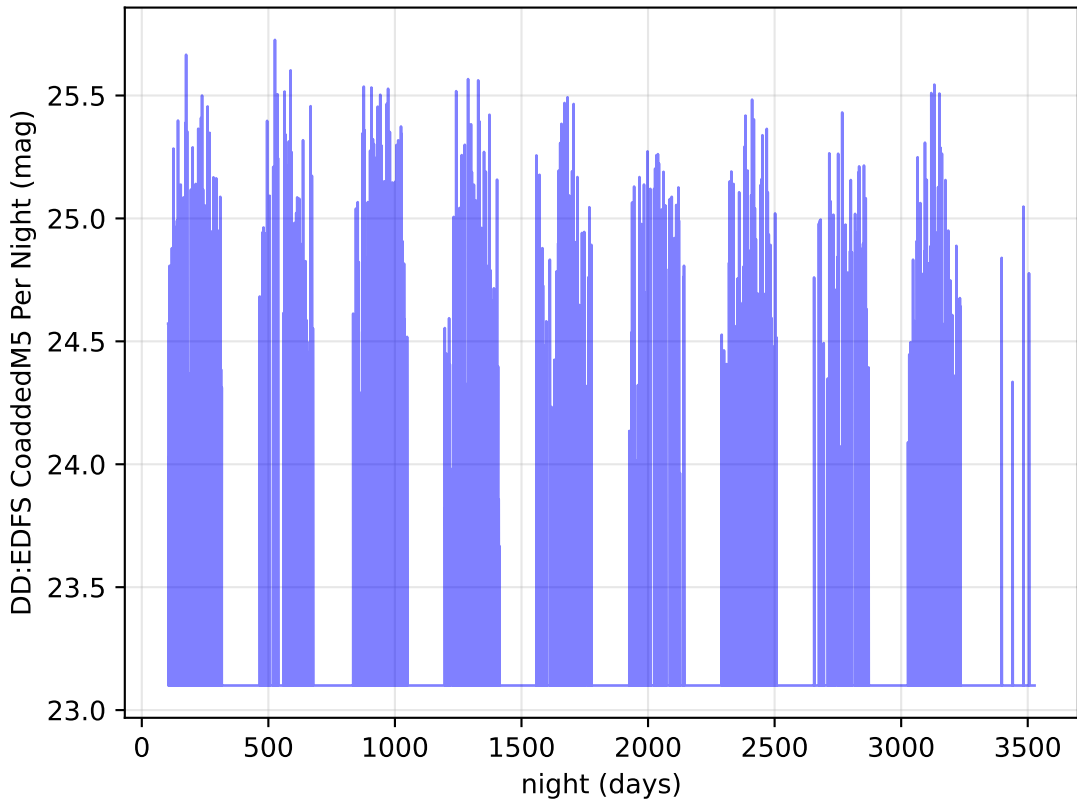
ddf_loaded_half_fl2_v3.4_10yrs i band: DD:EDFS CoaddedM5 Per Night
