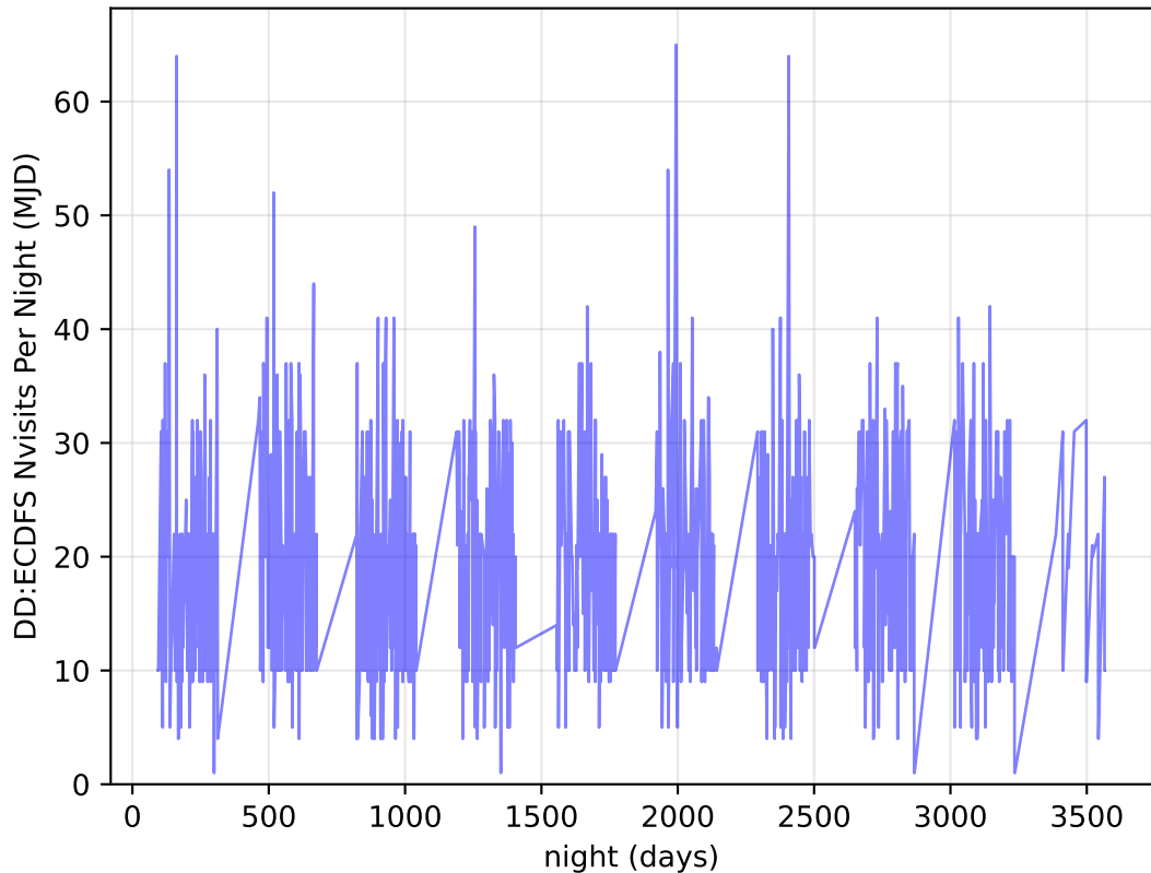
ddf_loaded_half_fl2_v3.4_10yrs all bands: DD:ECDFS Nvisits Per Night
