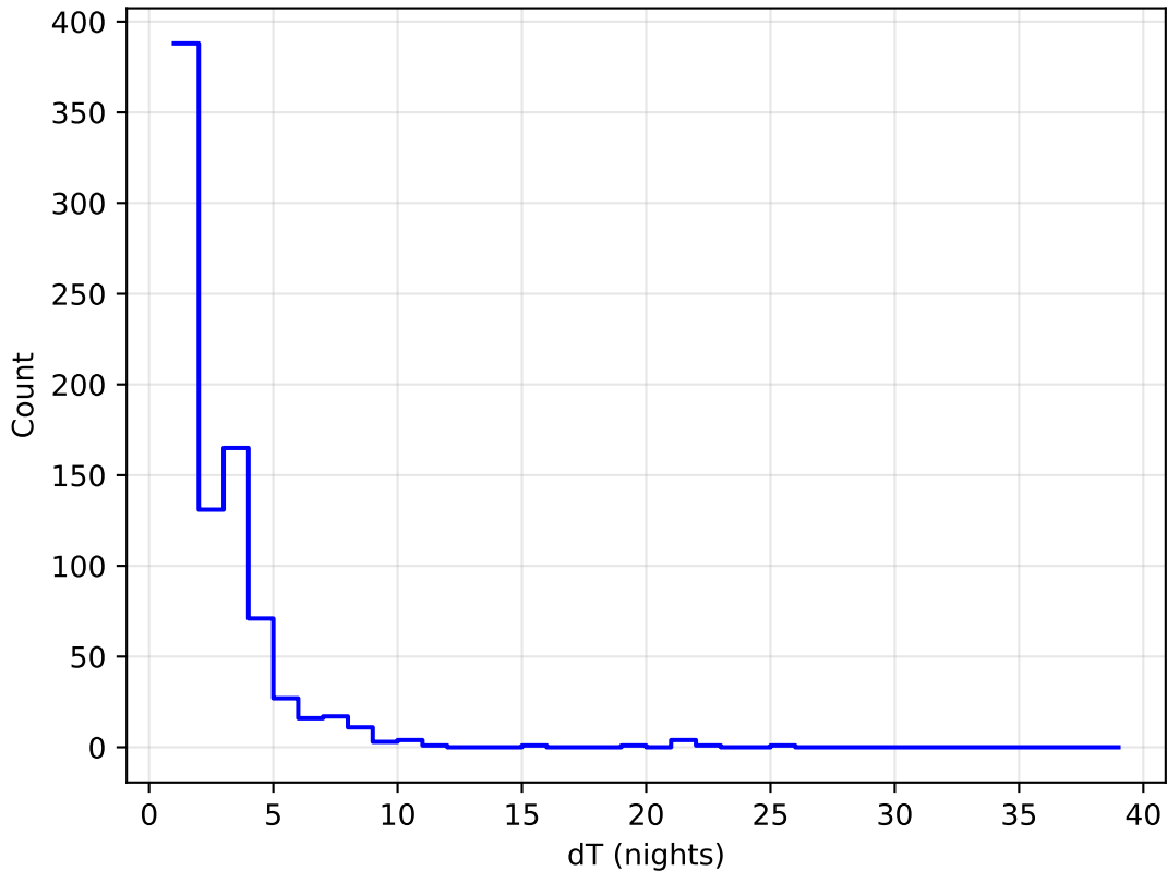
ddf_loaded_half_fl2_v3.4_10yrs all bands: DD:ECDFS Delta Nights Histogram
