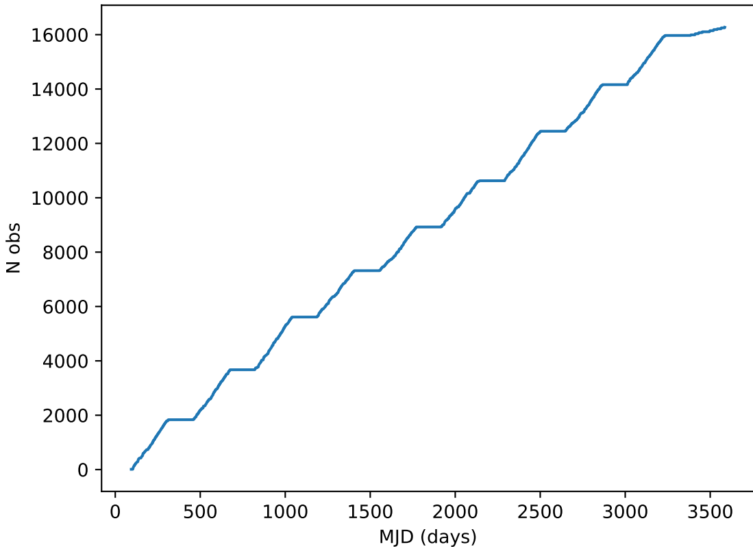
ddf_loaded_half_fl2_v3.4_10yrs all bands: DD:ECDFS Cumulative NVisits
