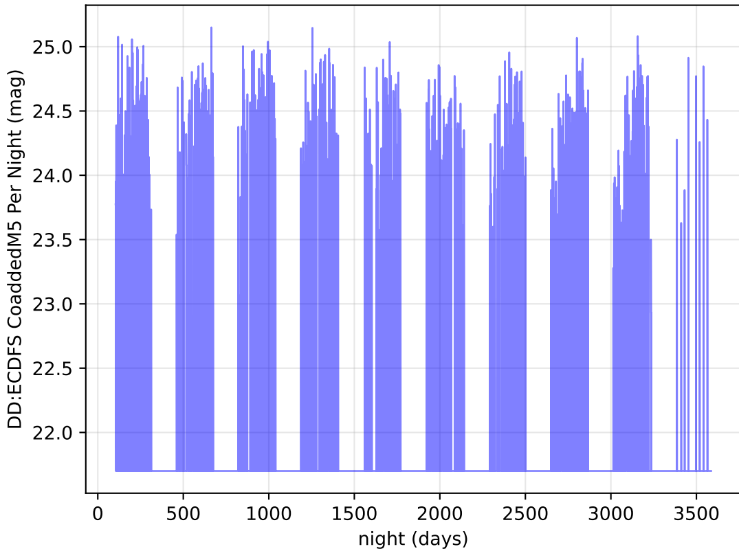
ddf_loaded_half_fl2_v3.4_10yrs z band: DD:ECDFS CoaddedM5 Per Night
