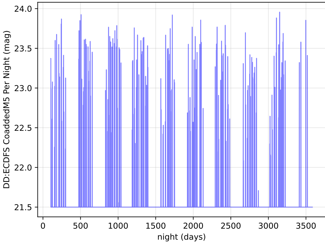
ddf_loaded_half_fi2_v3.4_10yrs y band: DD:ECDFS CoaddedM5 Per Night
