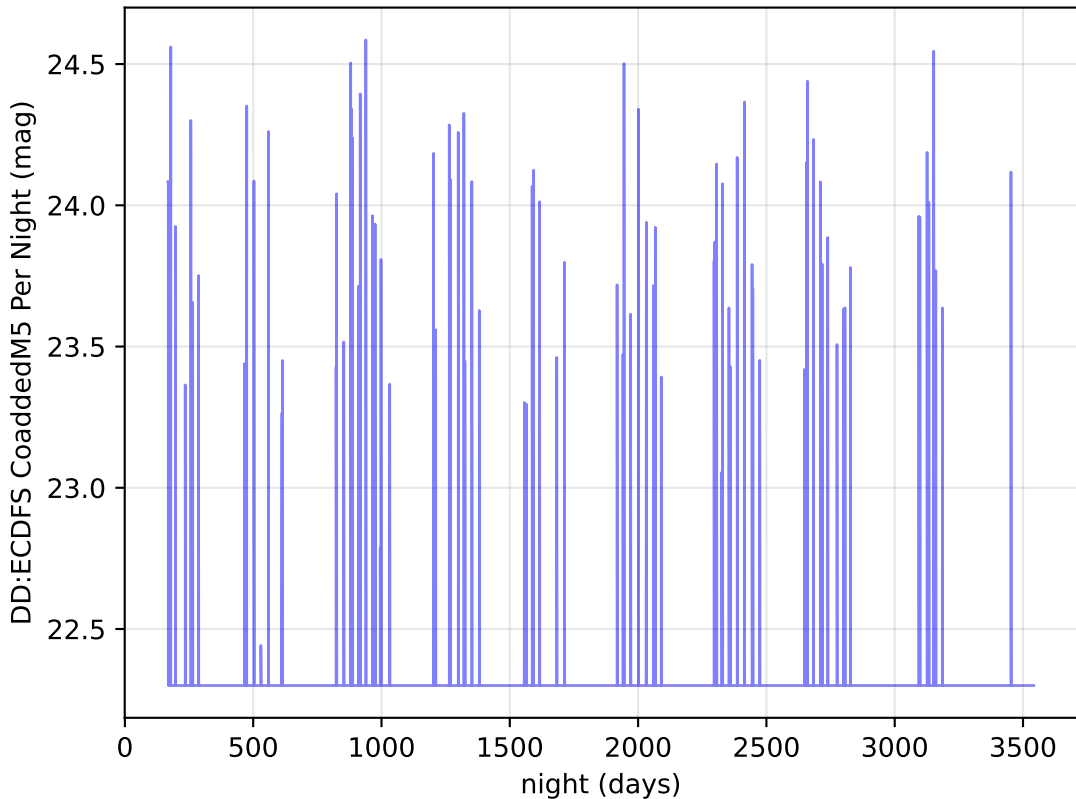
ddf_loaded_half_fl2_v3.4_10yrs u band: DD:ECDFS CoaddedM5 Per Night
