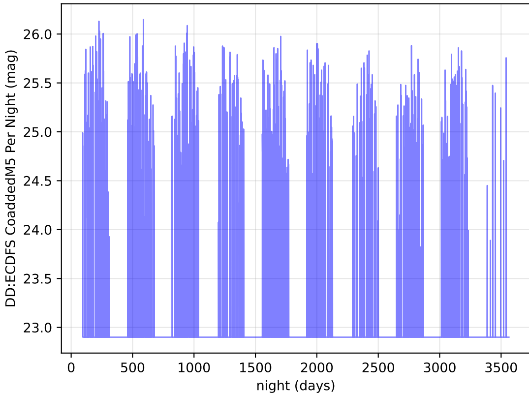
ddf_loaded_half_fl2_v3.4_10yrs r band: DD:ECDFS CoaddedM5 Per Night
