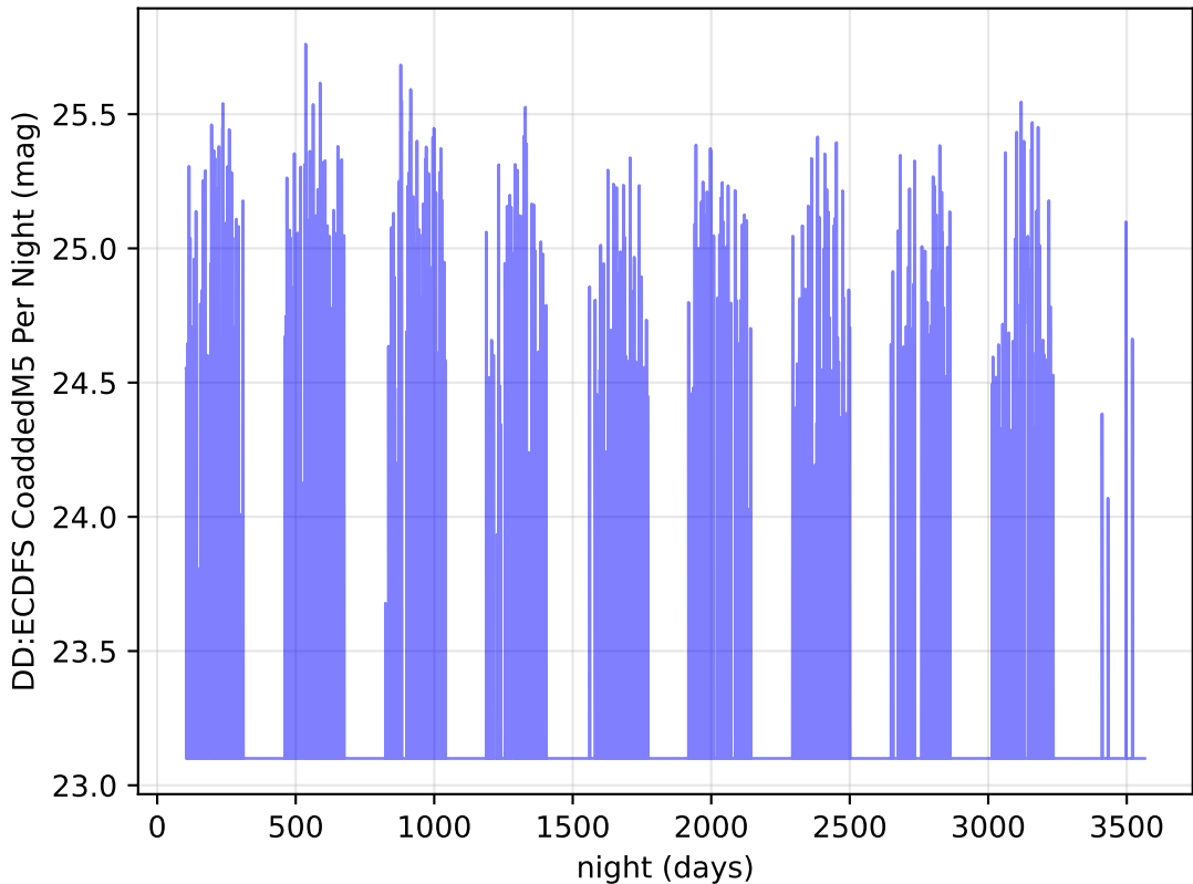
ddf_loaded_half_fl2_v3.4_10yrs i band: DD:ECDFS CoaddedM5 Per Night
