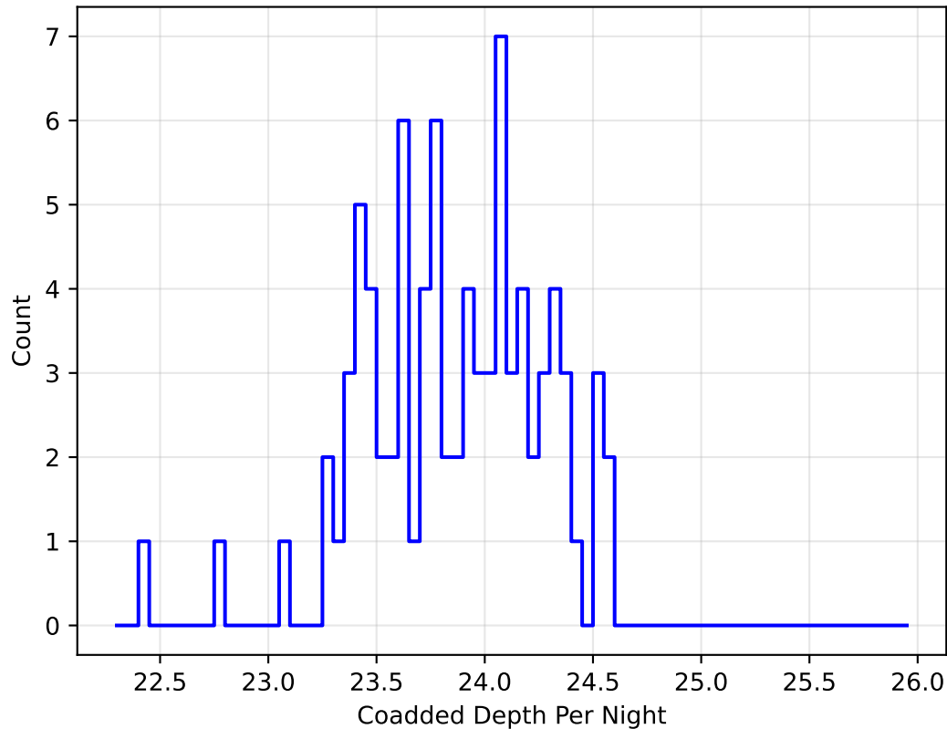
ddf_loaded_half_fl2_v3.4_10yrs u band: DD:ECDFS CoaddM5PerNight
