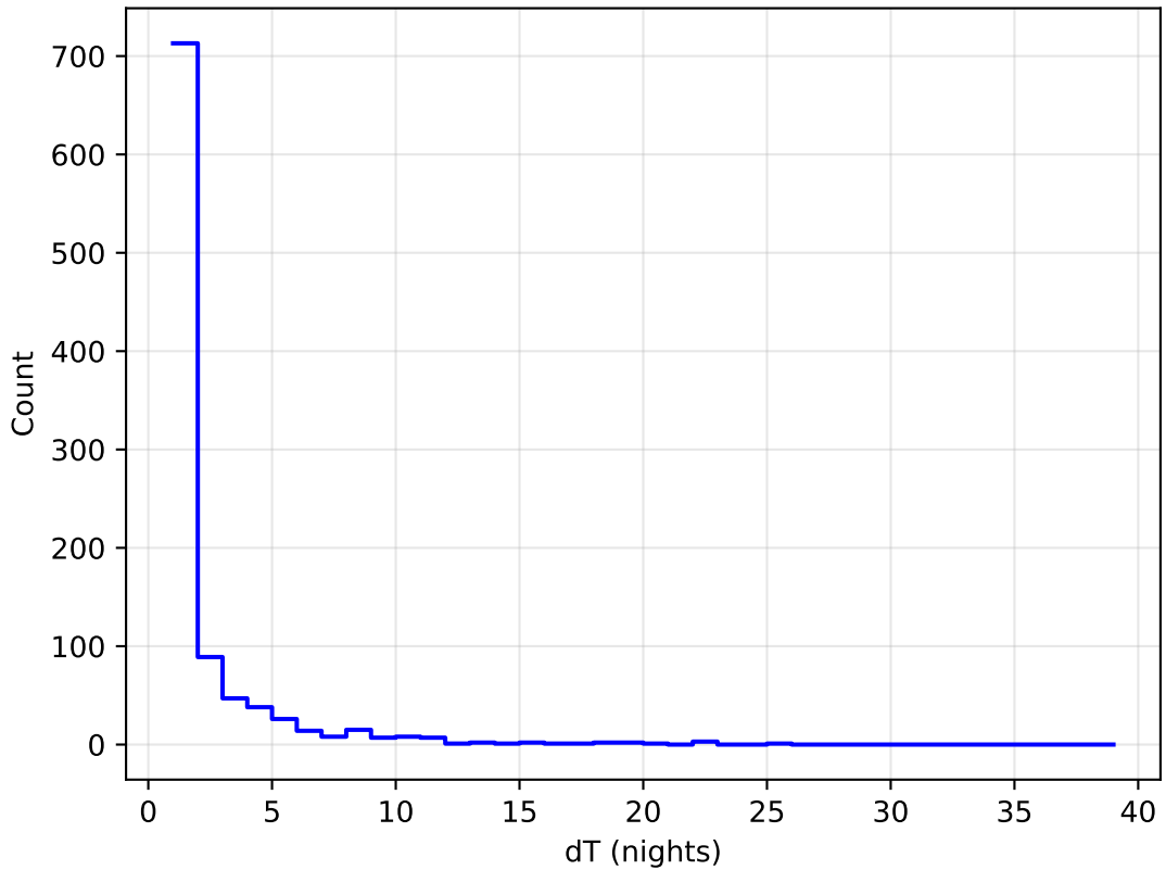
ddf_loaded_half_fl2_v3.4_10yrs all bands: DD: COSMOS Delta Nights Histogram
