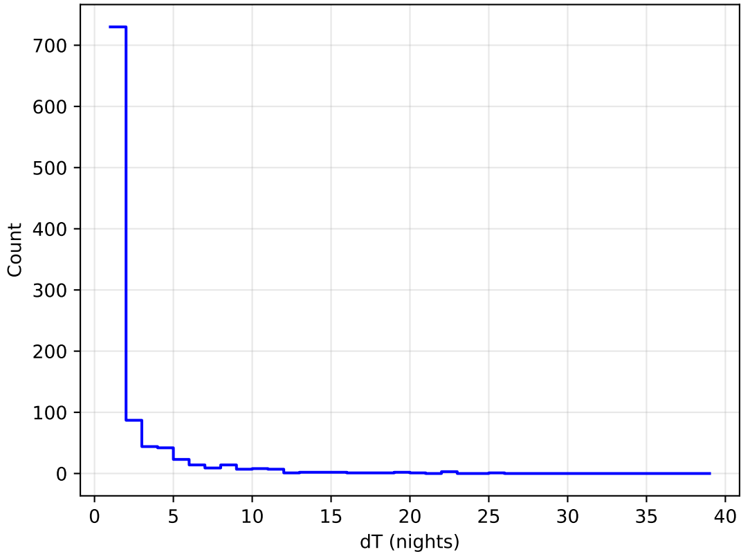
ddf_loaded_half_fl2_v3.4_10yrs all bands: DD:COSMOS Delta Nights Histogram
