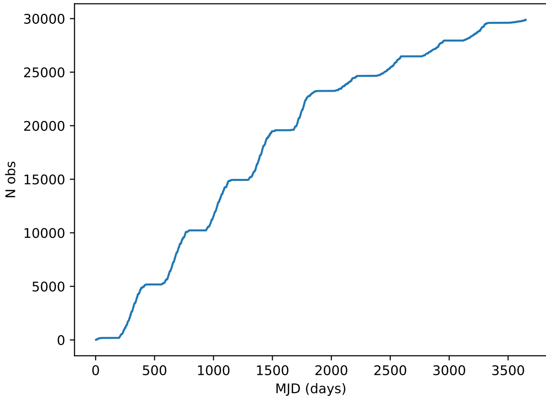
ddf_loaded_half_fl2_v3.4_10yrs all bands: DD: COSMOS Cumulative NVisits
