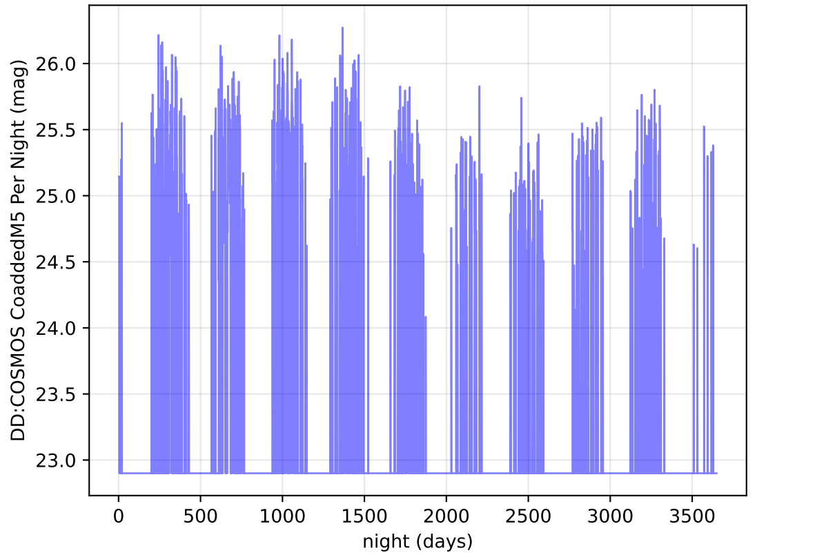
ddf_loaded_half_fl2_v3.4_10yrs r band: DD:COSMOS CoaddedM5 Per Night
