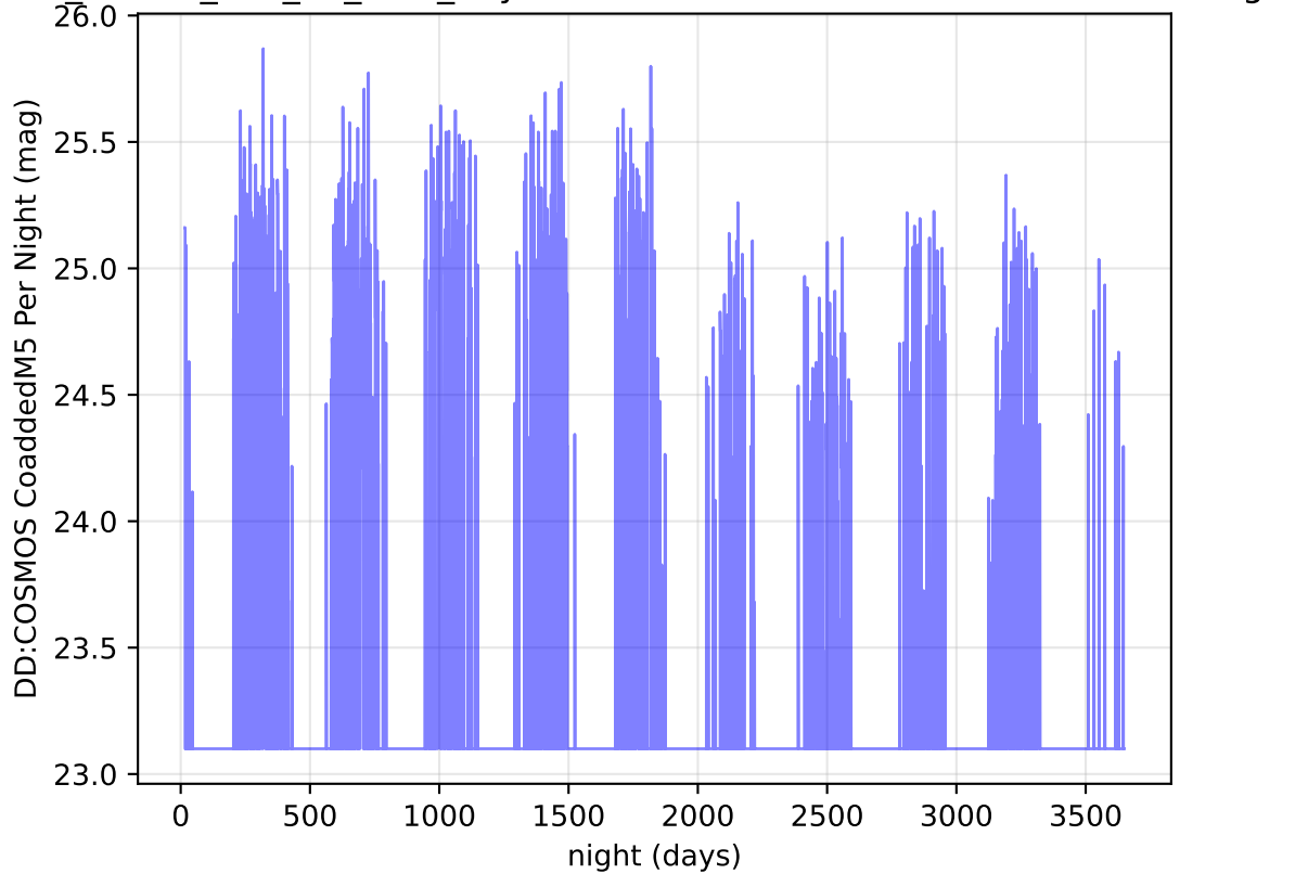
ddf_loaded_half_fl2_v3.4_10yrs i band: DD:COSMOS CoaddedM5 Per Night
