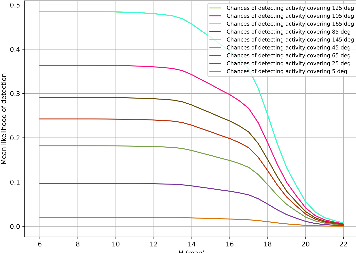
ddf loaded half fl1 v3.4 10yrs OCC r5
