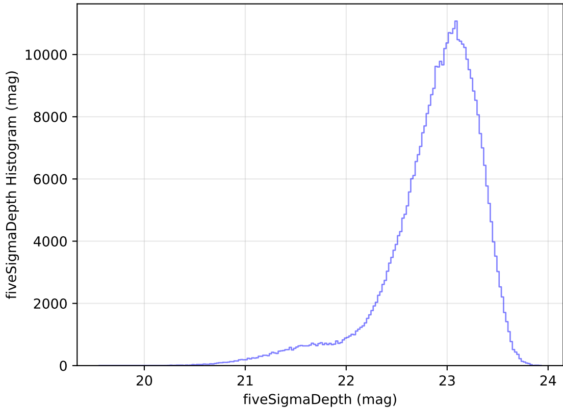
ddf_loaded_half_fl1_v3.4_10yrs z: fiveSigmaDepth Histogram
