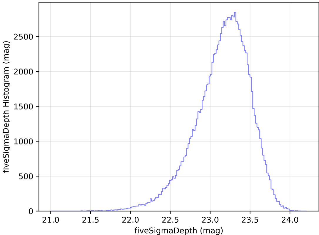
ddf_loaded_half_fl1_v3.4_10yrs u: fiveSigmaDepth Histogram
