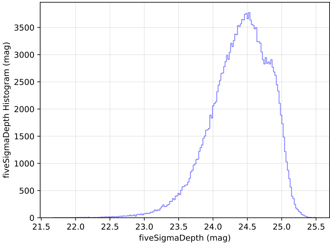
ddf_loaded_half_fl1_v3.4_10yrs g: fiveSigmaDepth Histogram
