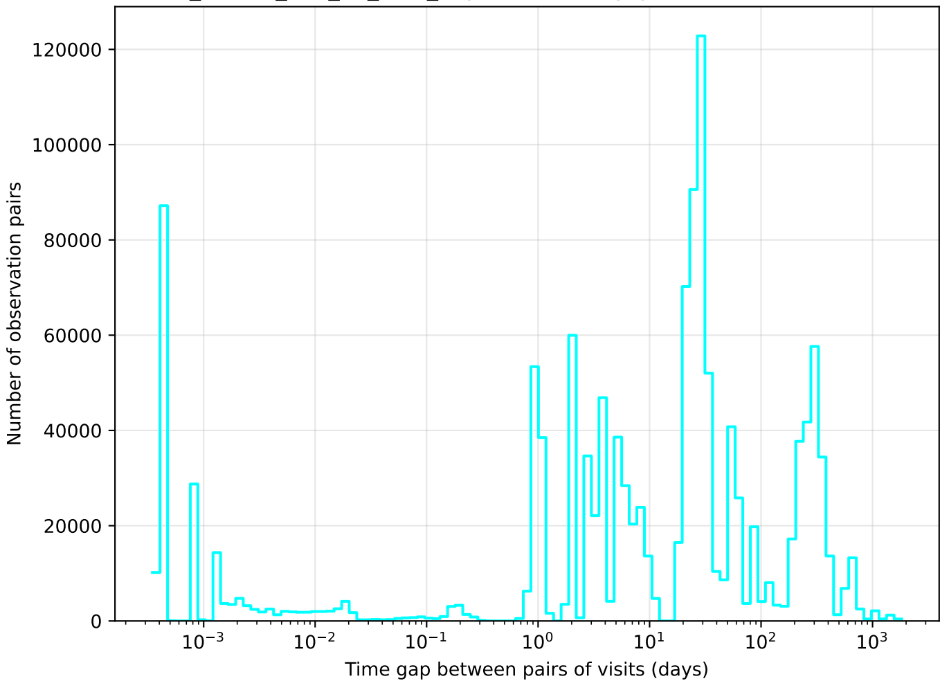
ddf_loaded_half_fl1_v3.4_10yrs u band: Tgaps observationStartMJD
