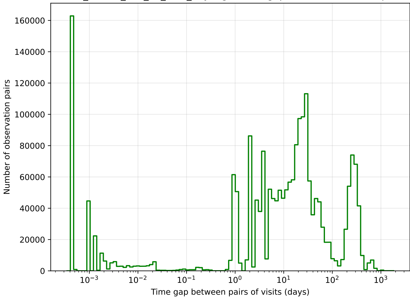
ddf_loaded_half_f11_v3.4_10yrs g band: Tgaps observationStartMJD
