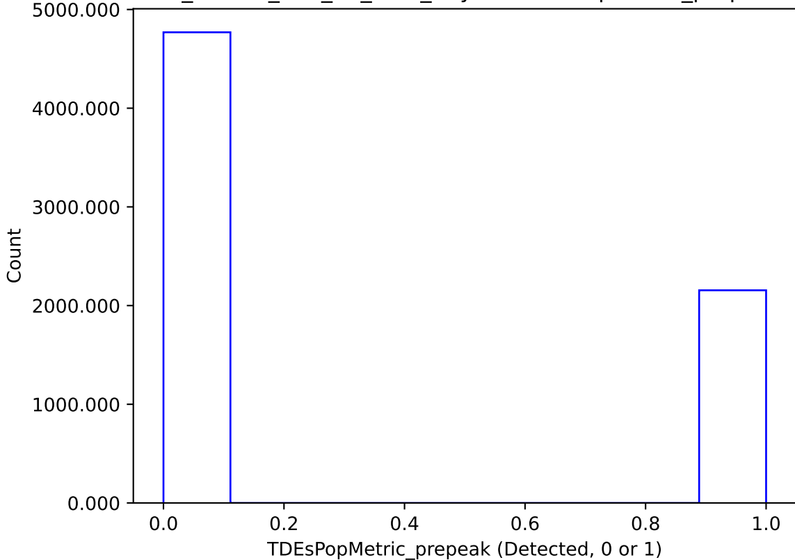
ddf_loaded_half_fl1_v3.4_10yrs : TDEsPopMetric_prepeak
