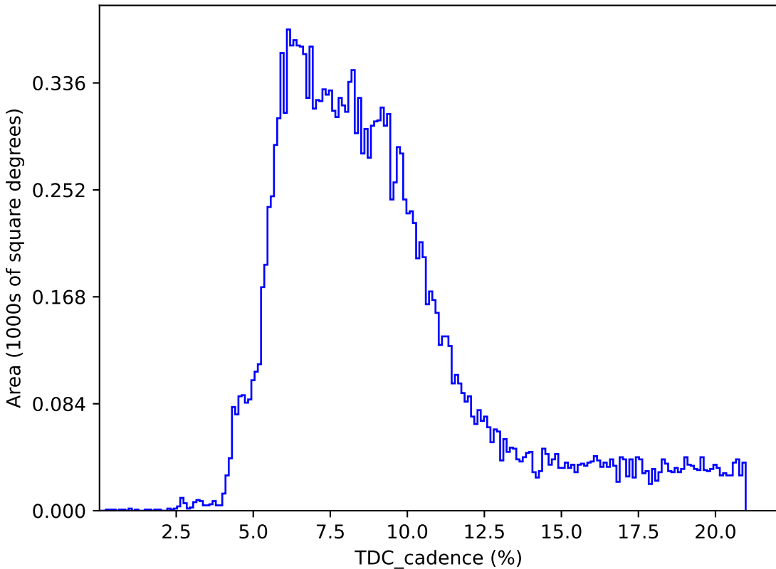
ddf_loaded_half_fl1_v3.4_10yrs : TDC_cadence
