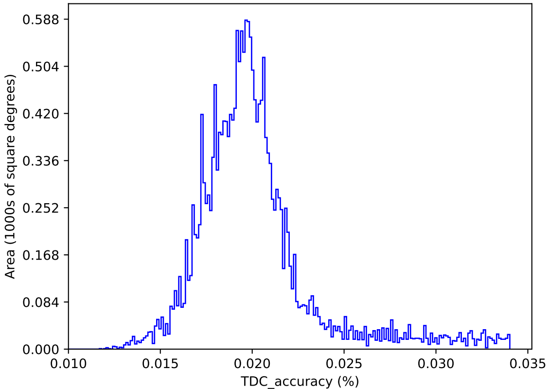
ddf_loaded_half_fl1_v3.4_10yrs : TDC_accuracy
