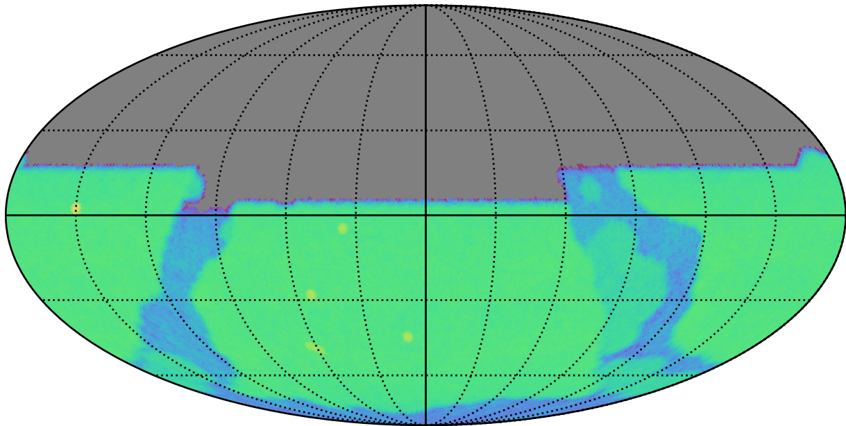
ddf_loaded_half_fl1_v3.4_10yrs u: SurfaceBrightLimit
