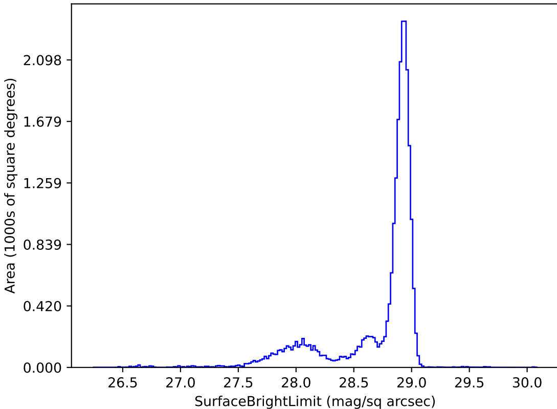
ddf_loaded_half_fl1_v3.4_10yrs u: SurfaceBrightLimit
