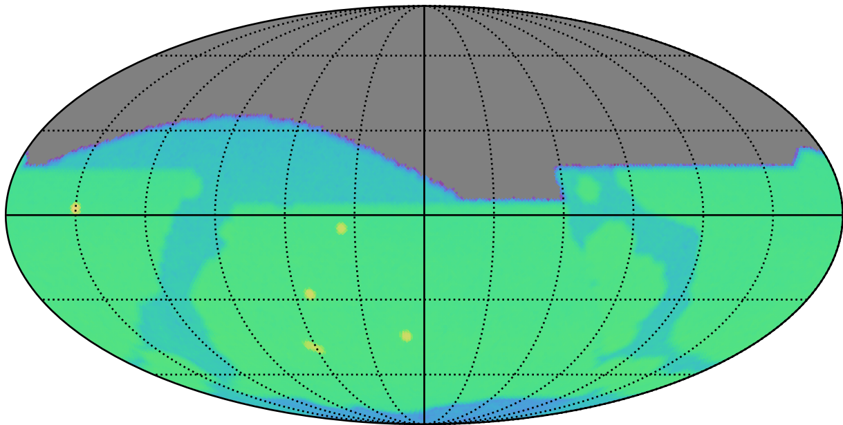
ddf_loaded_half_fl1_v3.4_10yrs r: SurfaceBrightLimit
