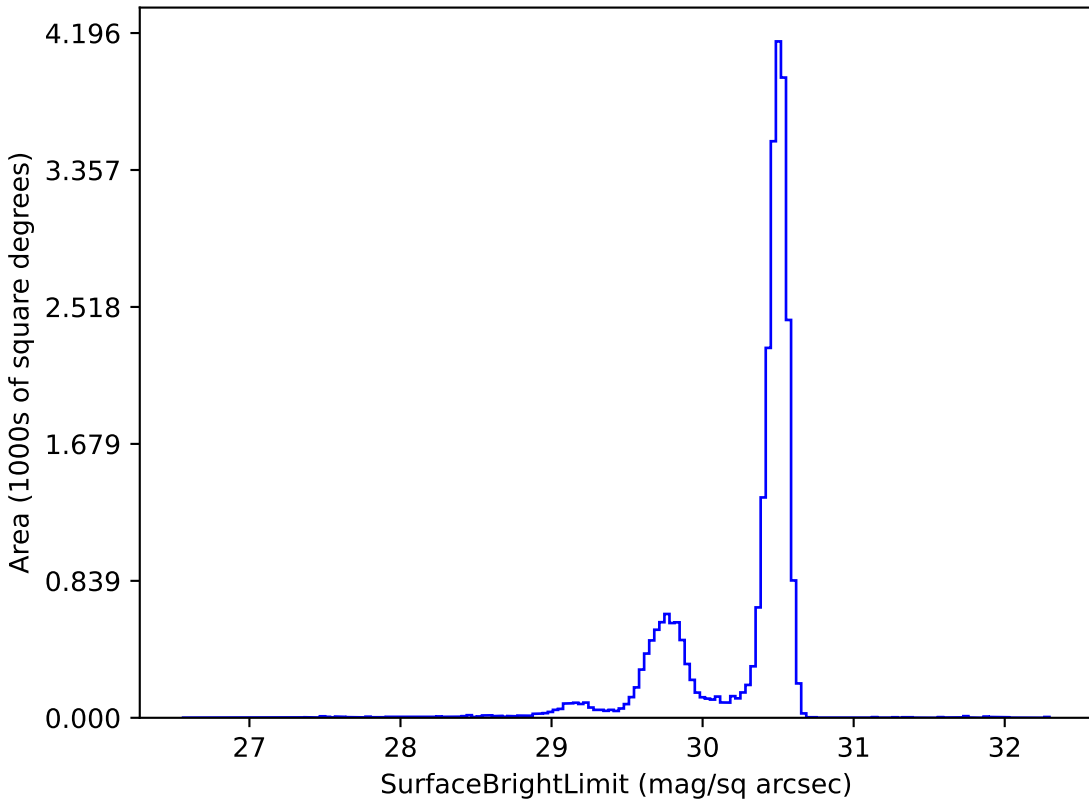
ddf_loaded_half_fl1_v3.4_10yrs r: SurfaceBrightLimit
