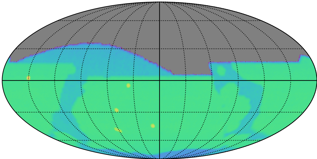
ddf_loaded_half_fl1_v3.4_10yrs i: SurfaceBrightLimit
