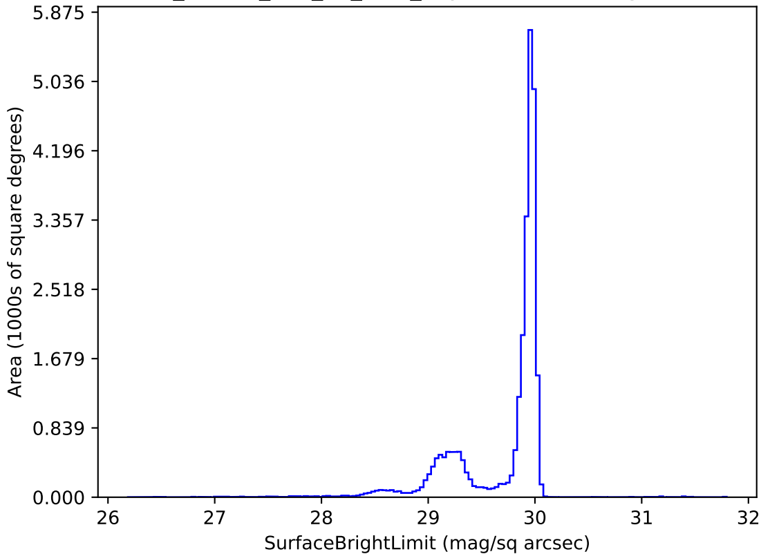
ddf_loaded_half_fl1_v3.4_10yrs i: SurfaceBrightLimit
