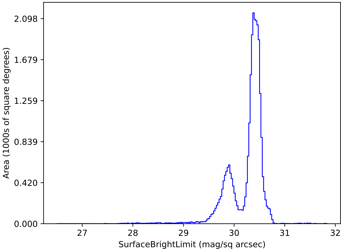
ddf_loaded_half_fl1_v3.4_10yrs g: SurfaceBrightLimit
