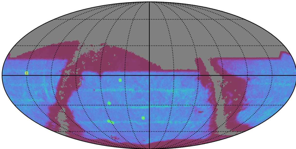
ddf_loaded_half_fl1_v3.4_10yrs : SNSLMetric
