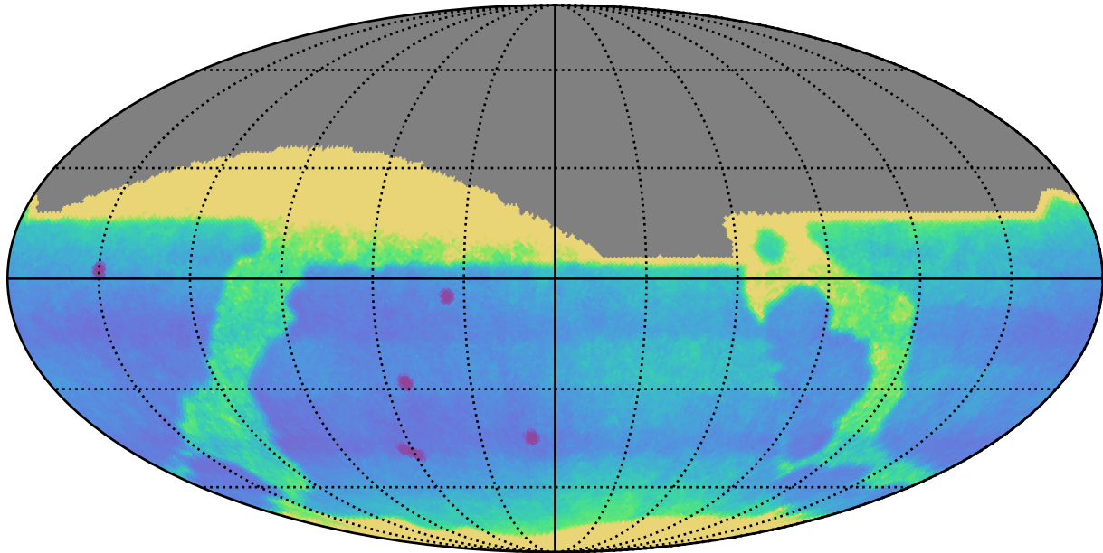
ddf_loaded_half_fl1_v3.4_10yrs : Proper Motion Uncert @ 24.0
