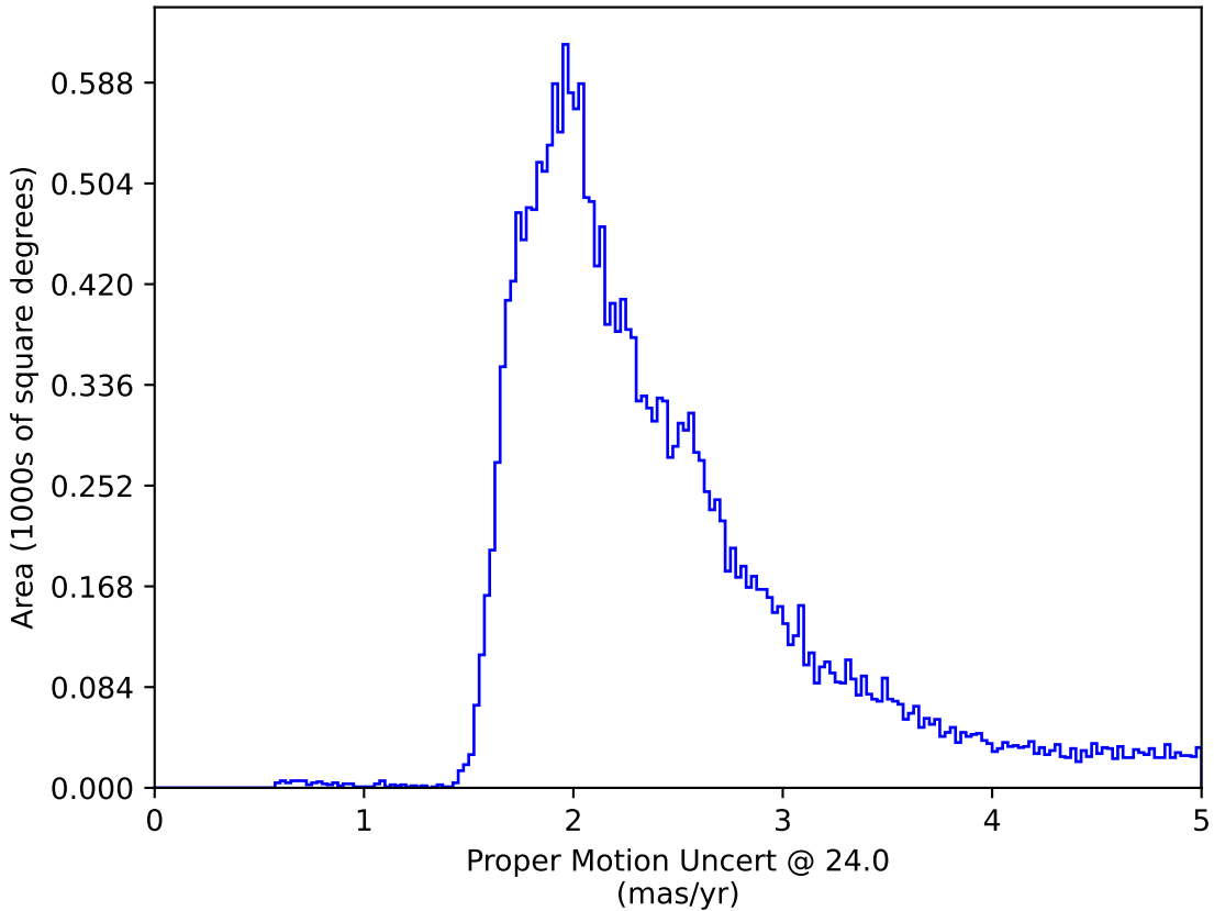
ddf_loaded_half_fl1_v3.4_10yrs : Proper Motion Uncert @ 24.0
