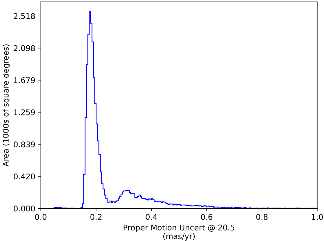
ddf_loaded_half_fl1_v3.4_10yrs : Proper Motion Uncert @ 20.5
