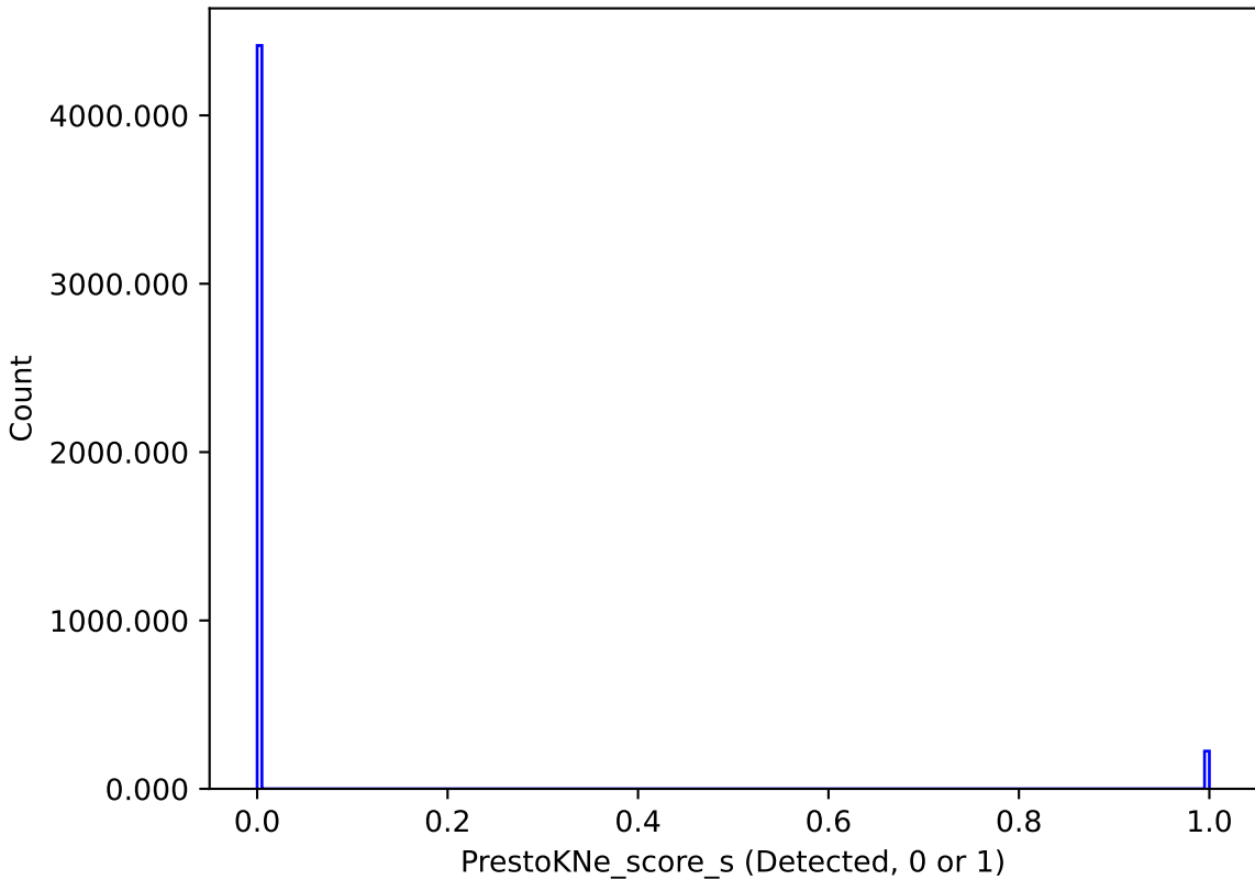
ddf_loaded_half_fl1_v3.4_10yrs : PrestoKNe_score_s
