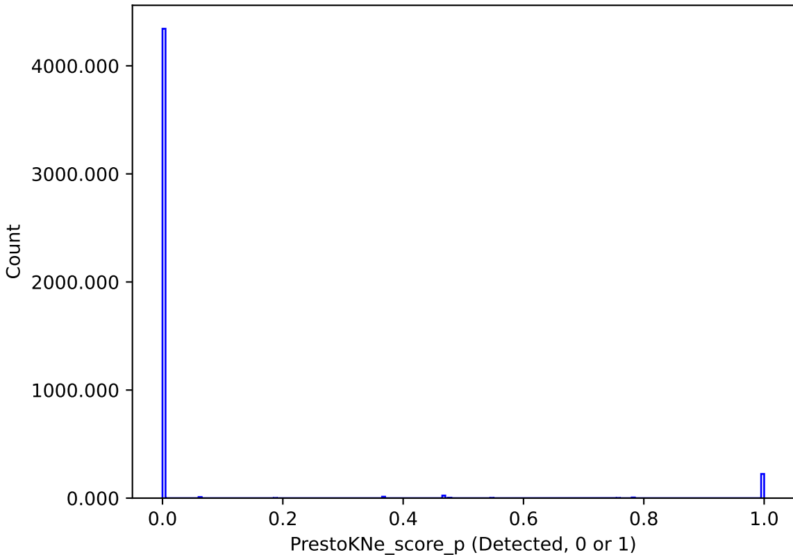
ddf_loaded_half_fl1_v3.4_10yrs : PrestoKNe_score_p
