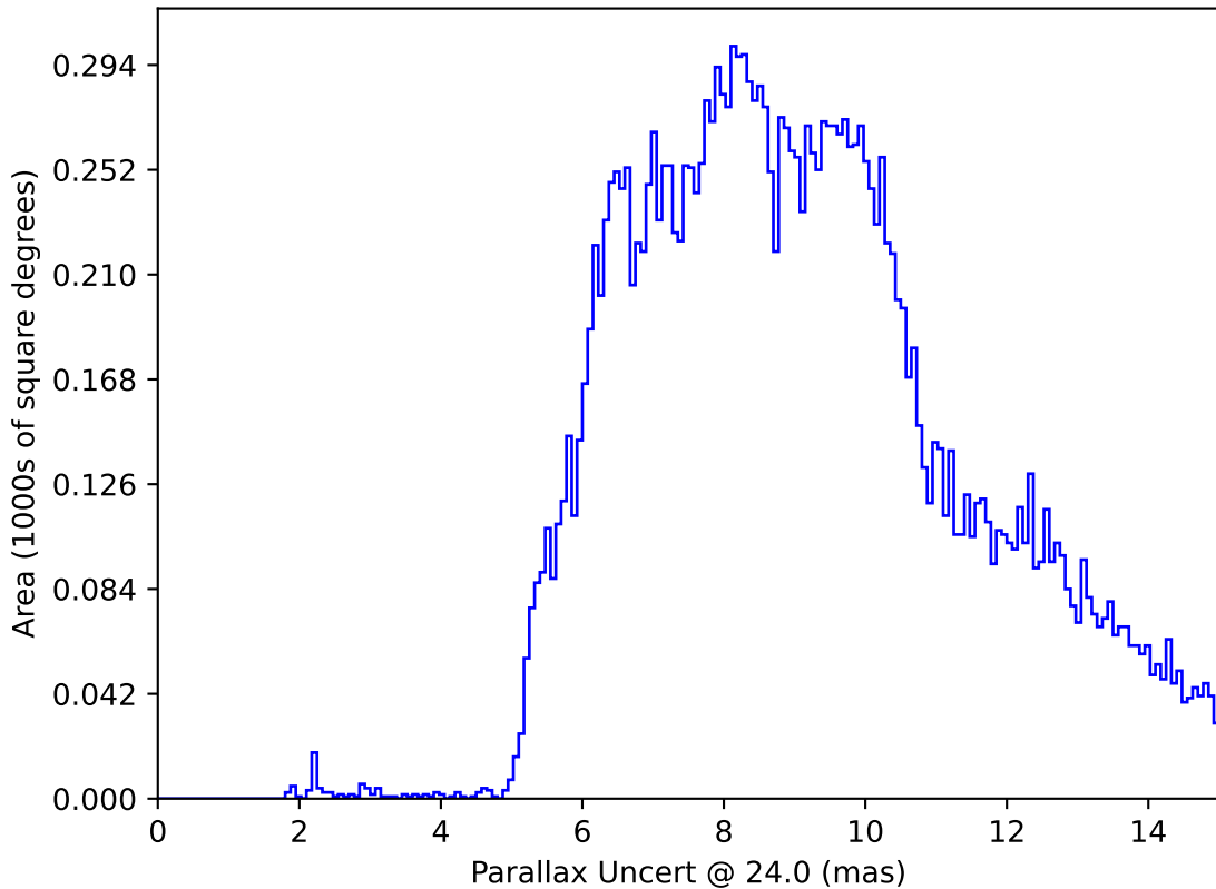
ddf_loaded_half_fl1_v3.4_10yrs : Parallax Uncert @ 24.0
