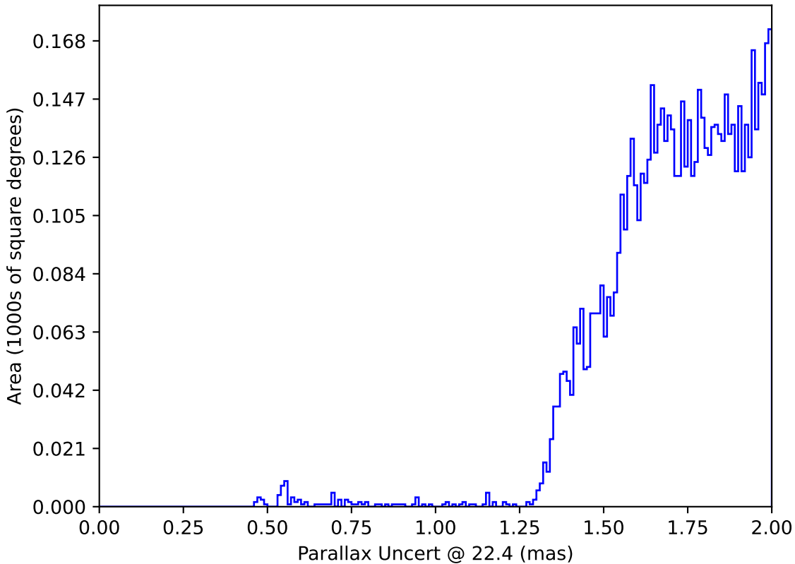
ddf_loaded_half_fl1_v3.4_10yrs : Parallax Uncert @ 22.4
