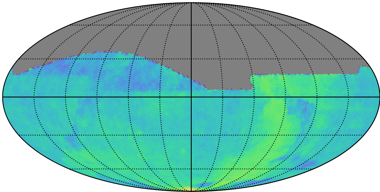
ddf_loaded_half_fl1_v3.4_10yrs : Parallax Coverage @ 24.0
