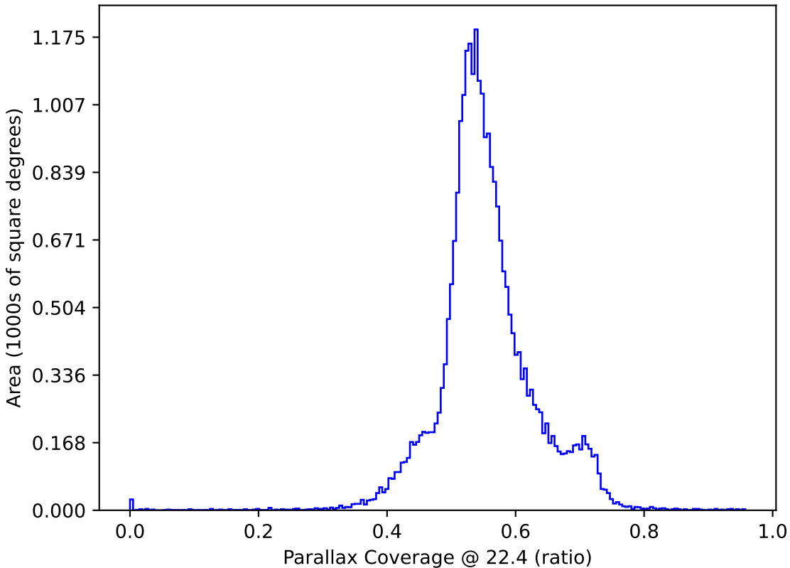
ddf_loaded_half_fl1_v3.4_10yrs : Parallax Coverage @ 22.4
