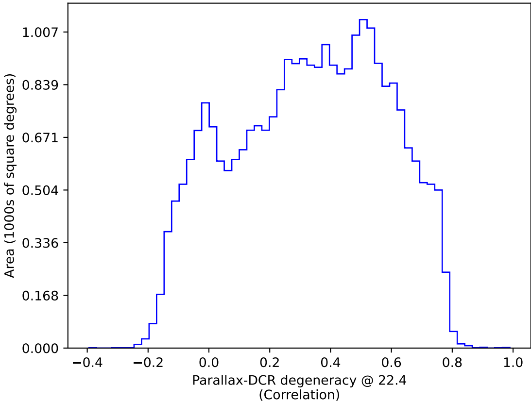
ddf_loaded_half_fl1_v3.4_10yrs : Parallax-DCR degeneracy @ 22.4
