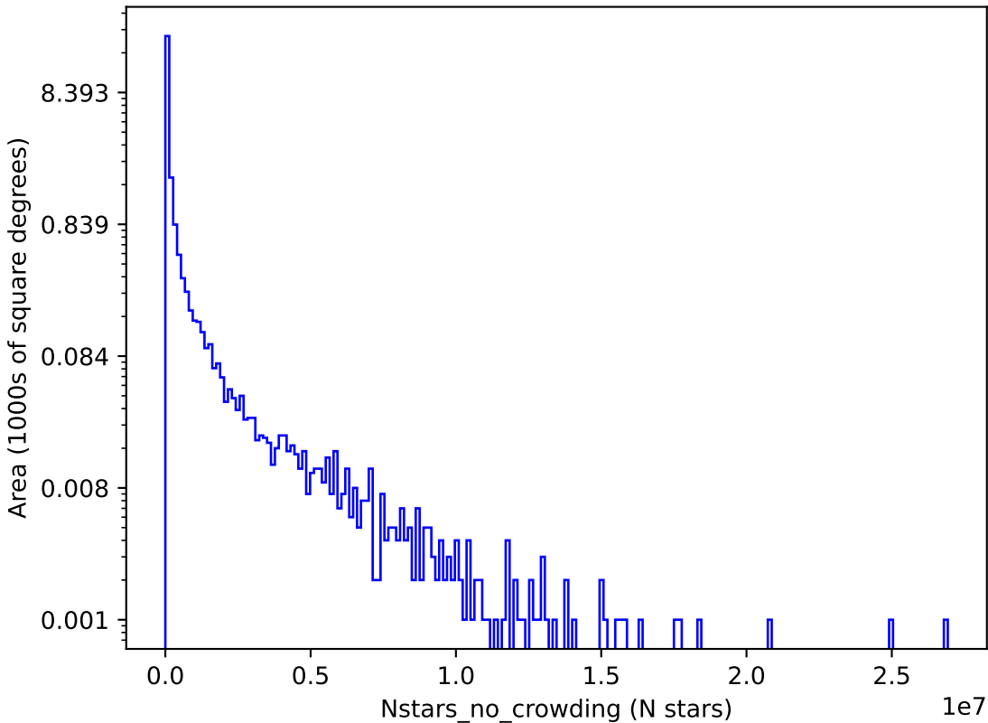
ddf_loaded_half_fl1_v3.4_10yrs z: Nstars_no_crowding
