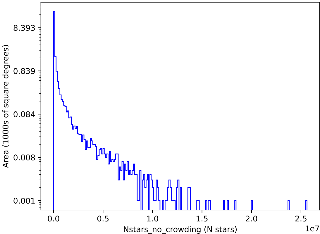
ddf_loaded_half_fl1_v3.4_10yrs y: Nstars_no_crowding
