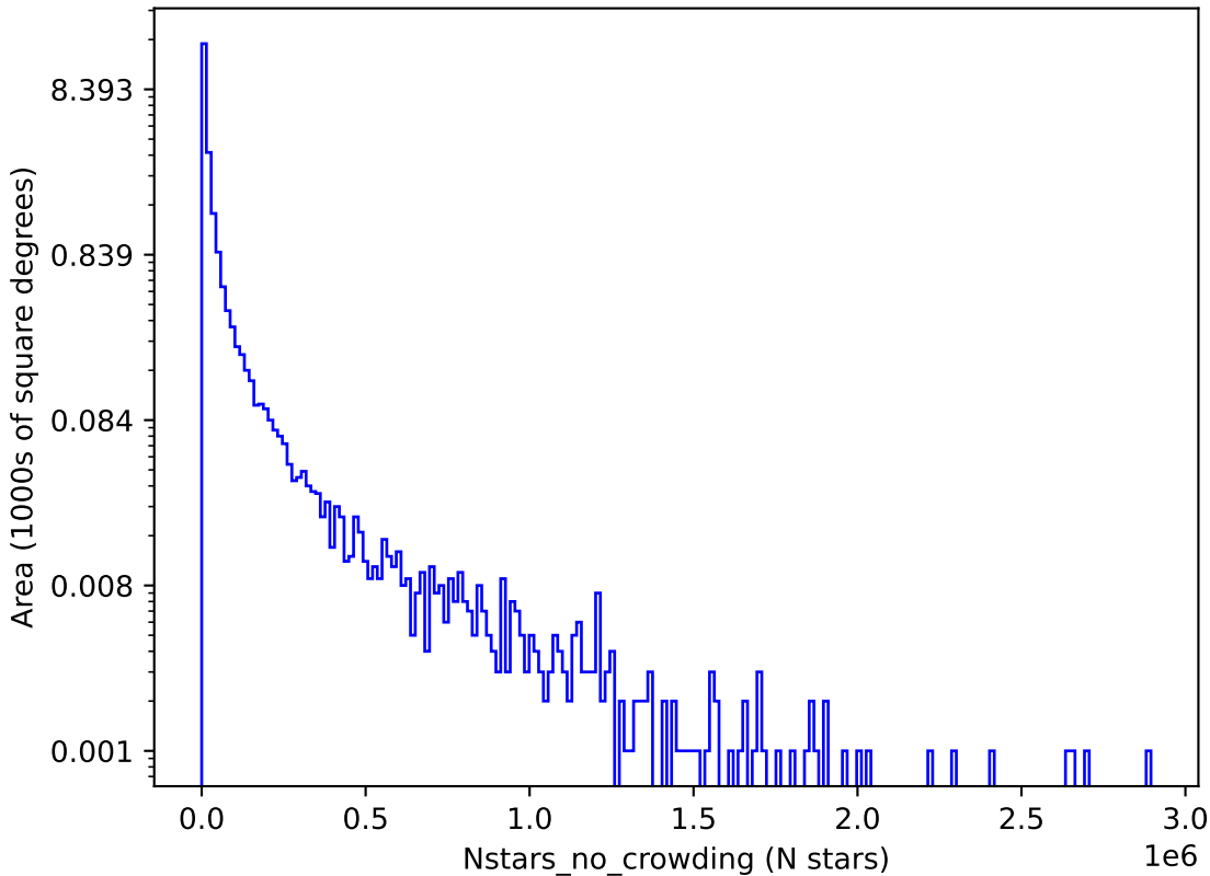
ddf_loaded_half_fl1_v3.4_10yrs u: Nstars_no_crowding
