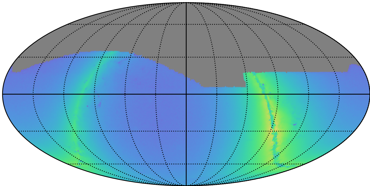
ddf_loaded_half_fl1_v3.4_10yrs r: Nstars_no_crowding
