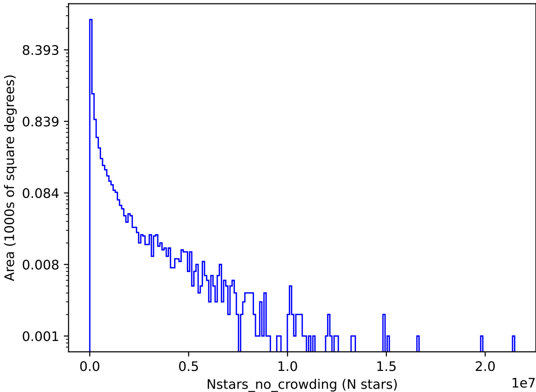
ddf_loaded_half_fl1_v3.4_10yrs r: Nstars_no_crowding
