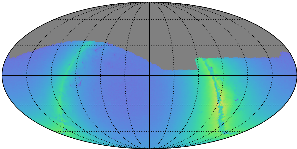
ddf_loaded_half_fl1_v3.4_10yrs g: Nstars_no_crowding
